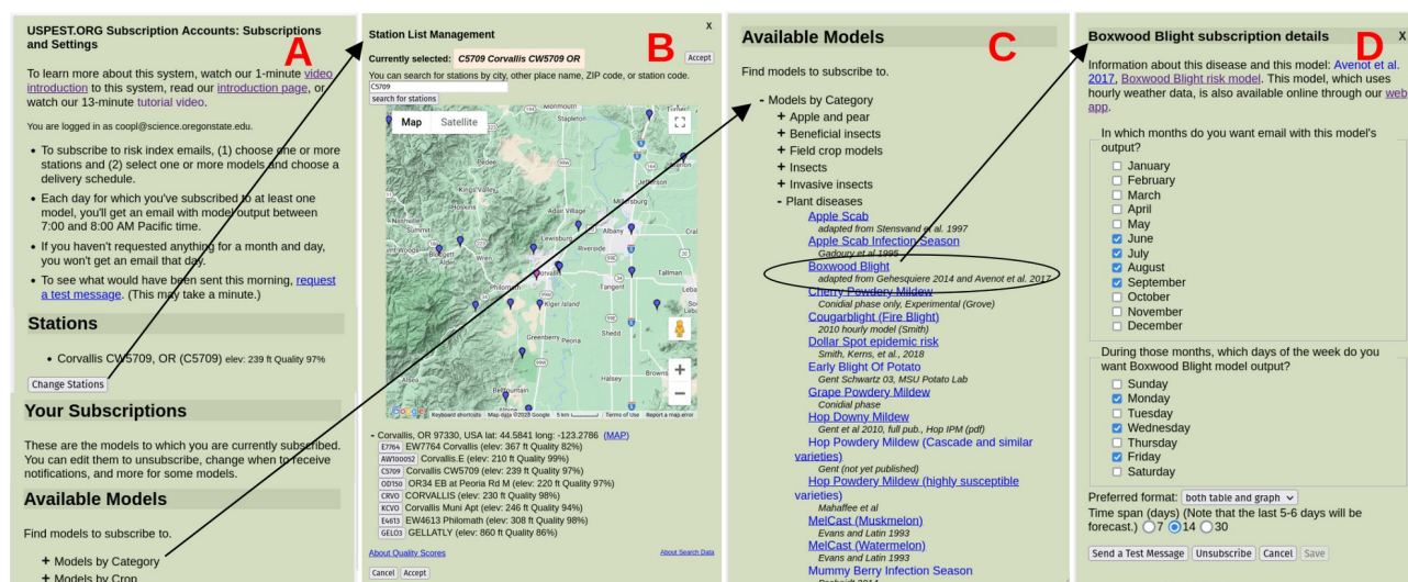
Fig. 2. Subscribing to boxwood blight model email “Push” notifications. This is similar to using the model itself for selection of weather stations (B and C). Select your schedule as shown (D).
